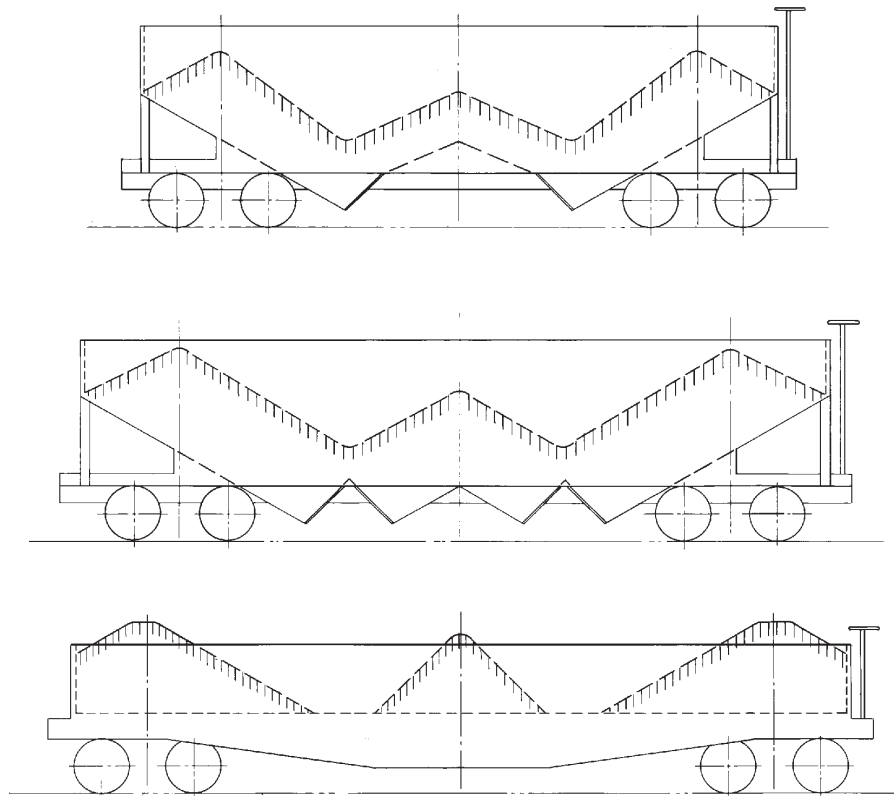
MANNER OF LOADING COAL AND COKE—HOPPER AND GONDOLA CARS. (Drawing Redrawn 9-1977)
