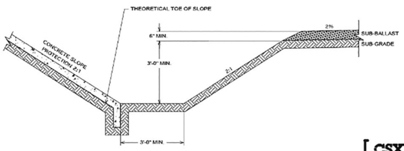
DITCH DETAIL
